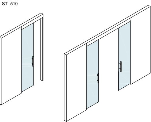
Pocket glass sliding doors
