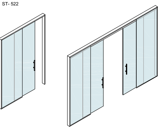
Pocket glass sliding doors into double butt glazed glass wall
